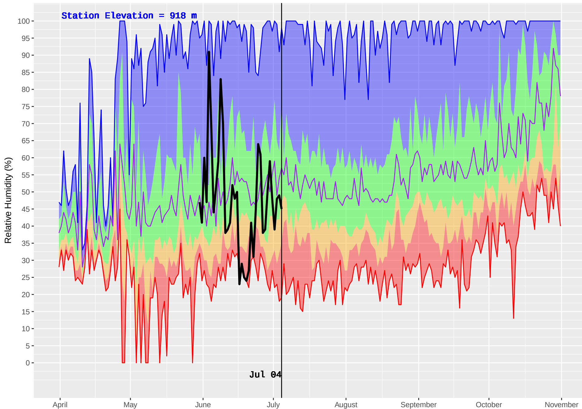
AUGIER LAKE (167) : Historical (1984–2016) and Current (2018) Noon Relative Humidity
