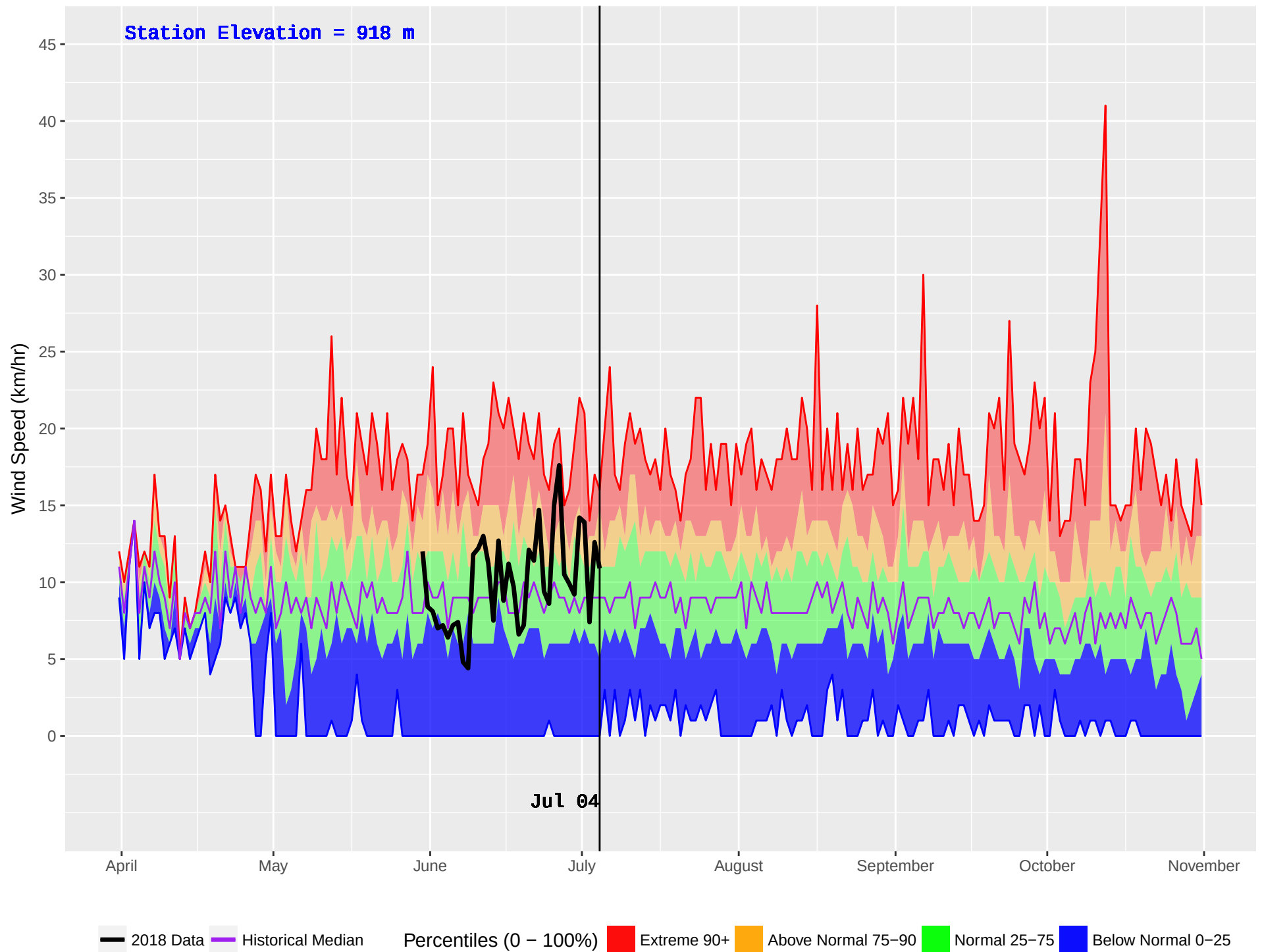
AUGIER LAKE (167) : Historical (1984–2016) and Current (2018) Noon Wind Speed
