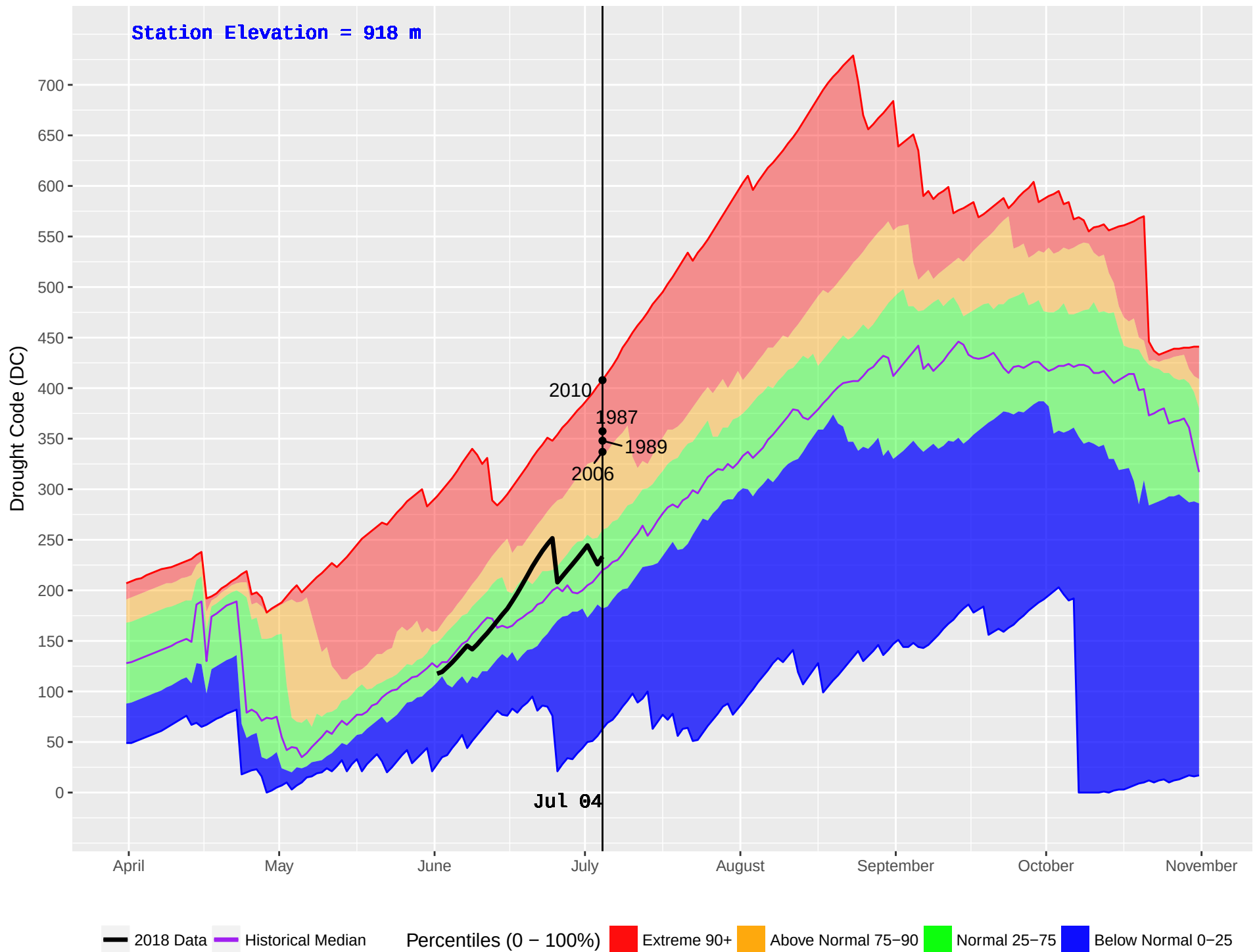
AUGIER LAKE (167) : Historical (1984–2016) and Current (2018) Noon Drought Code (DC)
