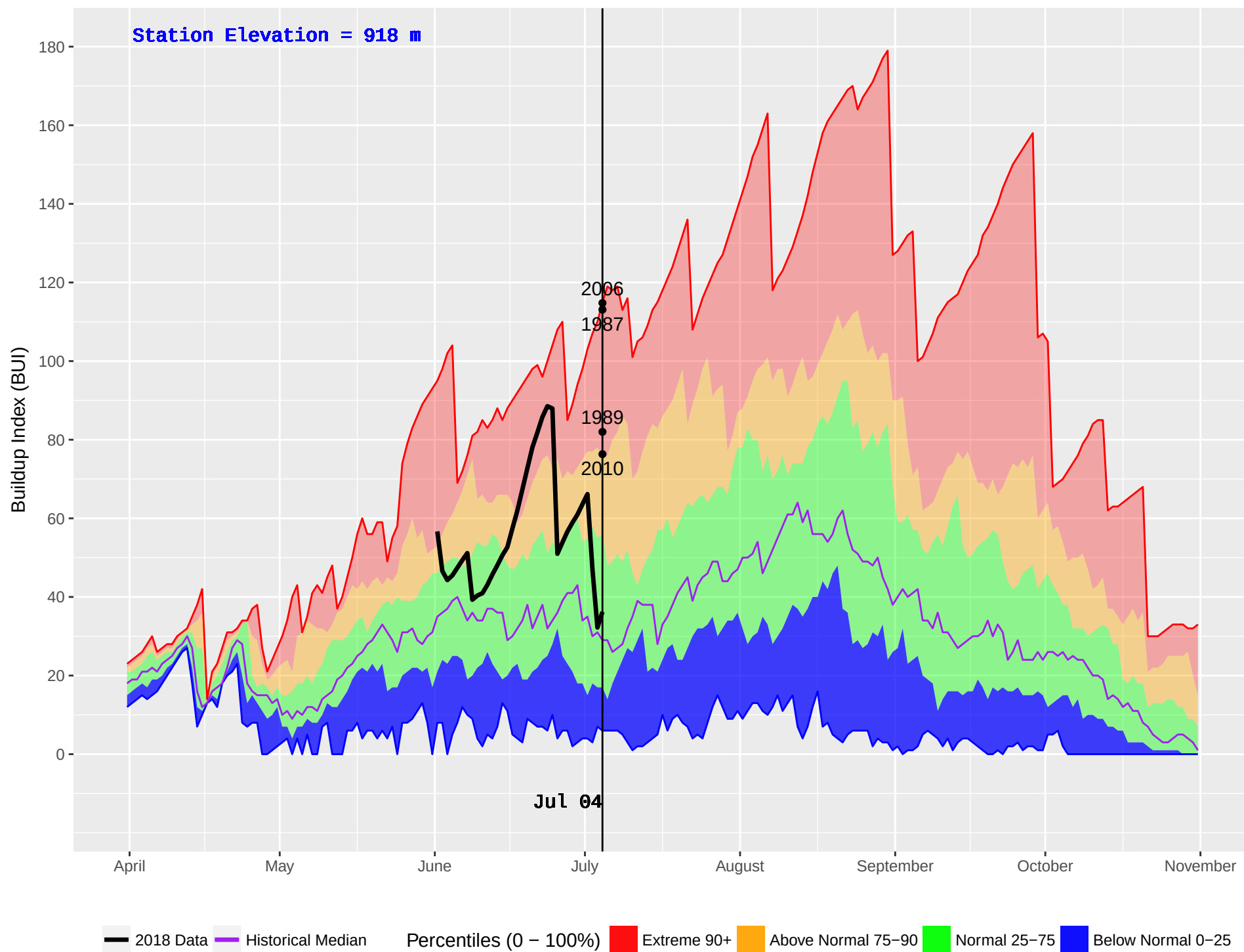
AUGIER LAKE (167) : Historical (1984–2016) and Current (2018) Noon Buildup Index (BUI)
