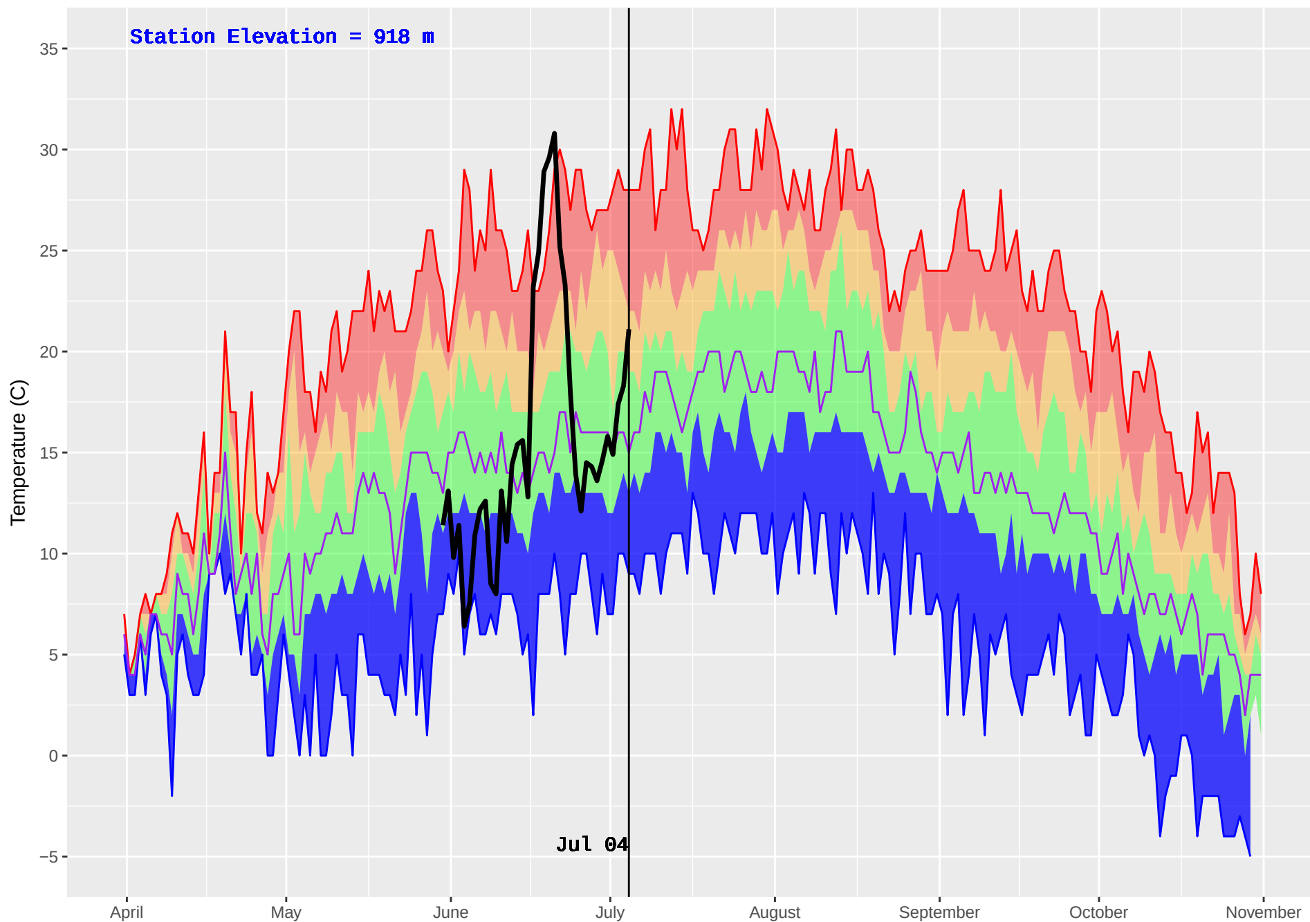
AUGIER LAKE (167) : Historical (1984–2016) and Current (2018) Noon Temperature
